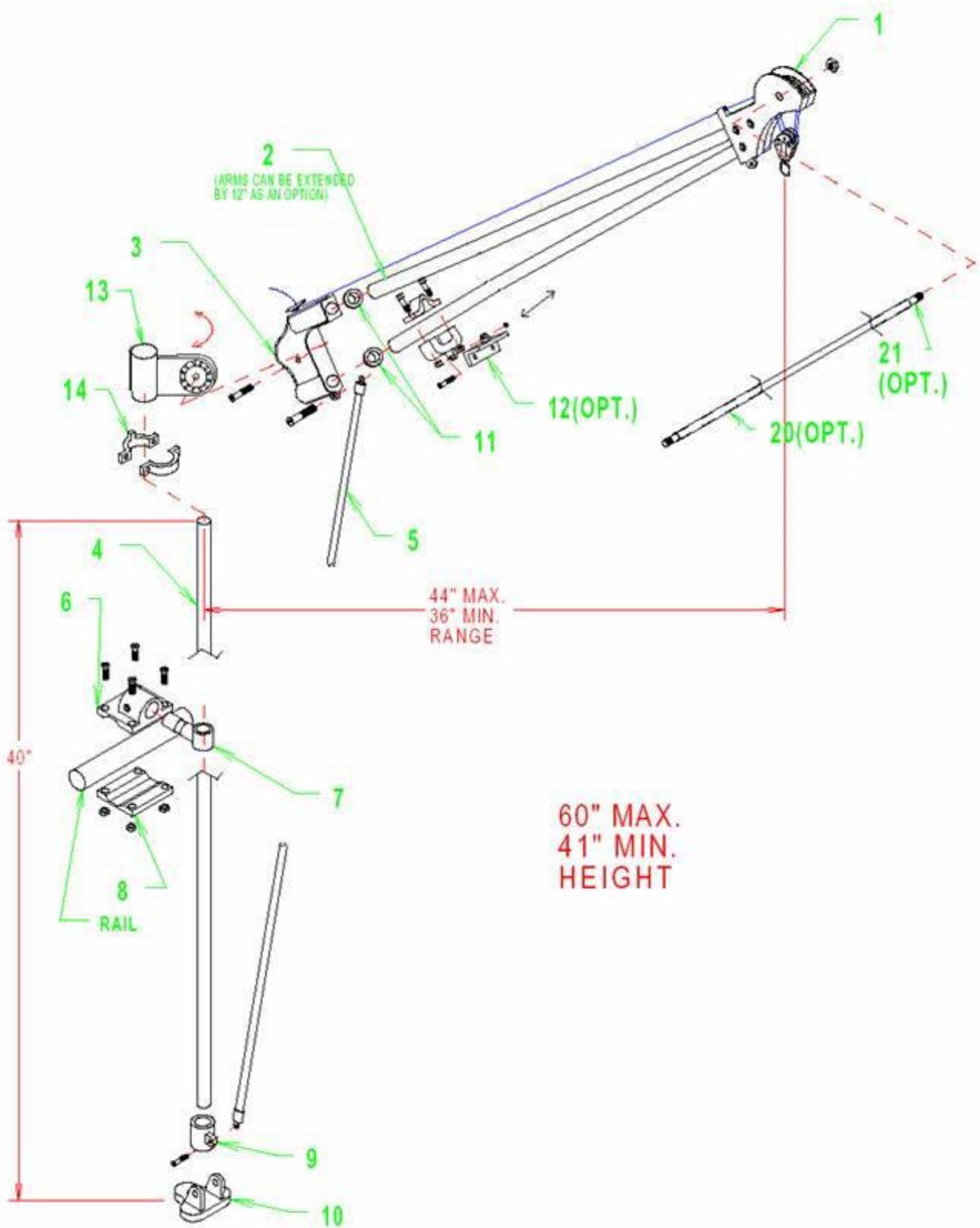
1900 Rotating Davit – Rail Mount Schematic
